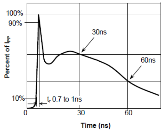
Fig.4 Pulse Waveform-ESD(IEC61000-4-2)
